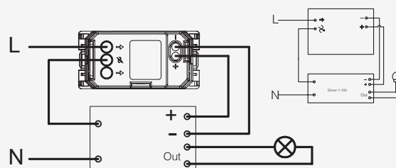
Dimmer 1-10V N0160.9 XX
